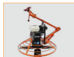
FOLDABLE AND HEIGHT ADJUSTABLE ARM
